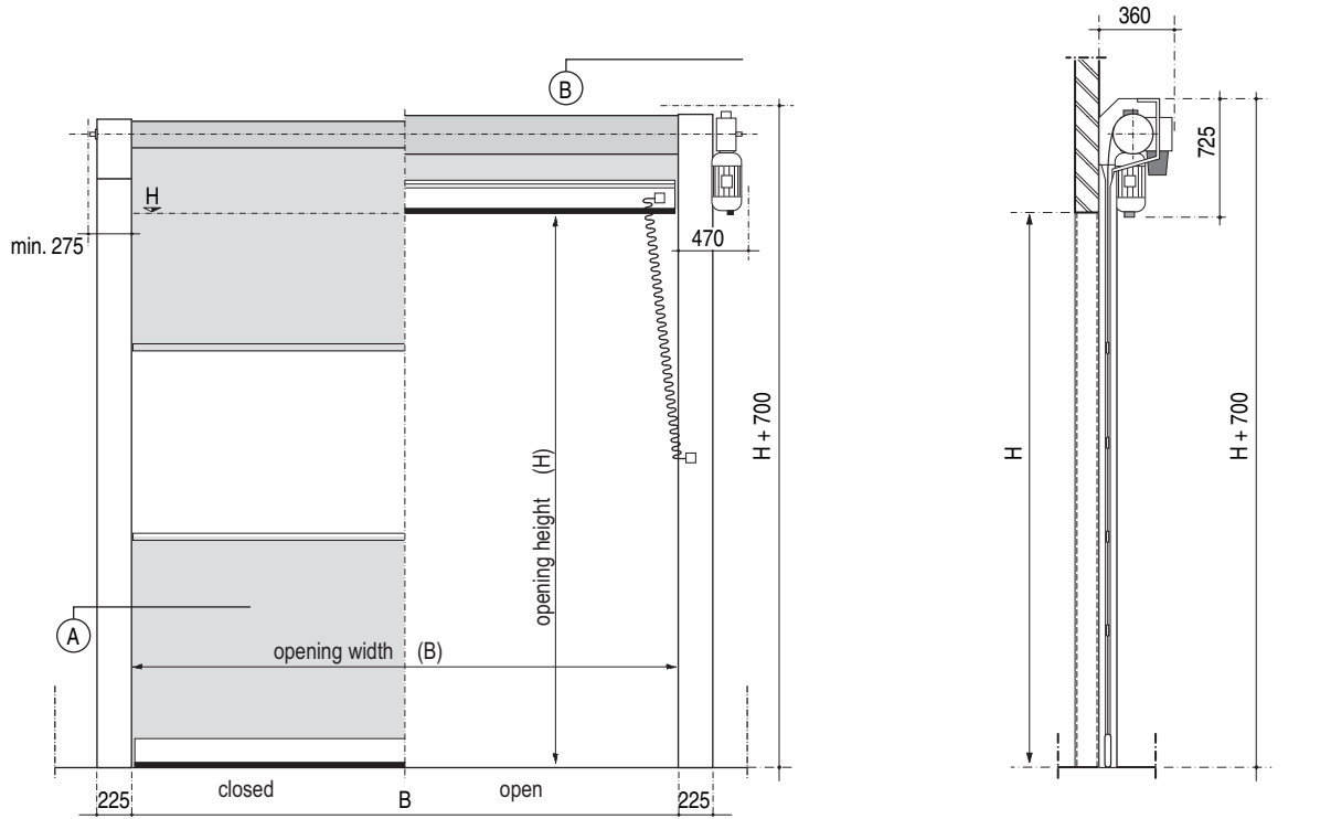
Front view
