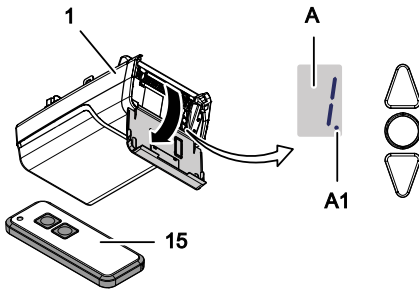
Fig. 4: Control elements
