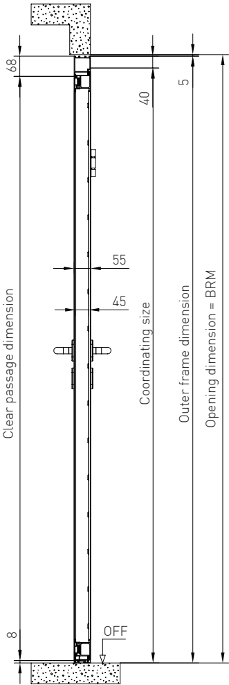
Vertical section/Installation in the opening
