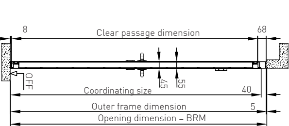
Horizontal section/Installation in the opening
