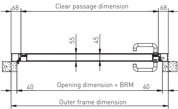
Horizontal section/Installation behind the opening
