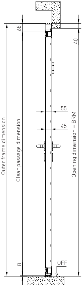
Horizontal section/Installation in the opening
